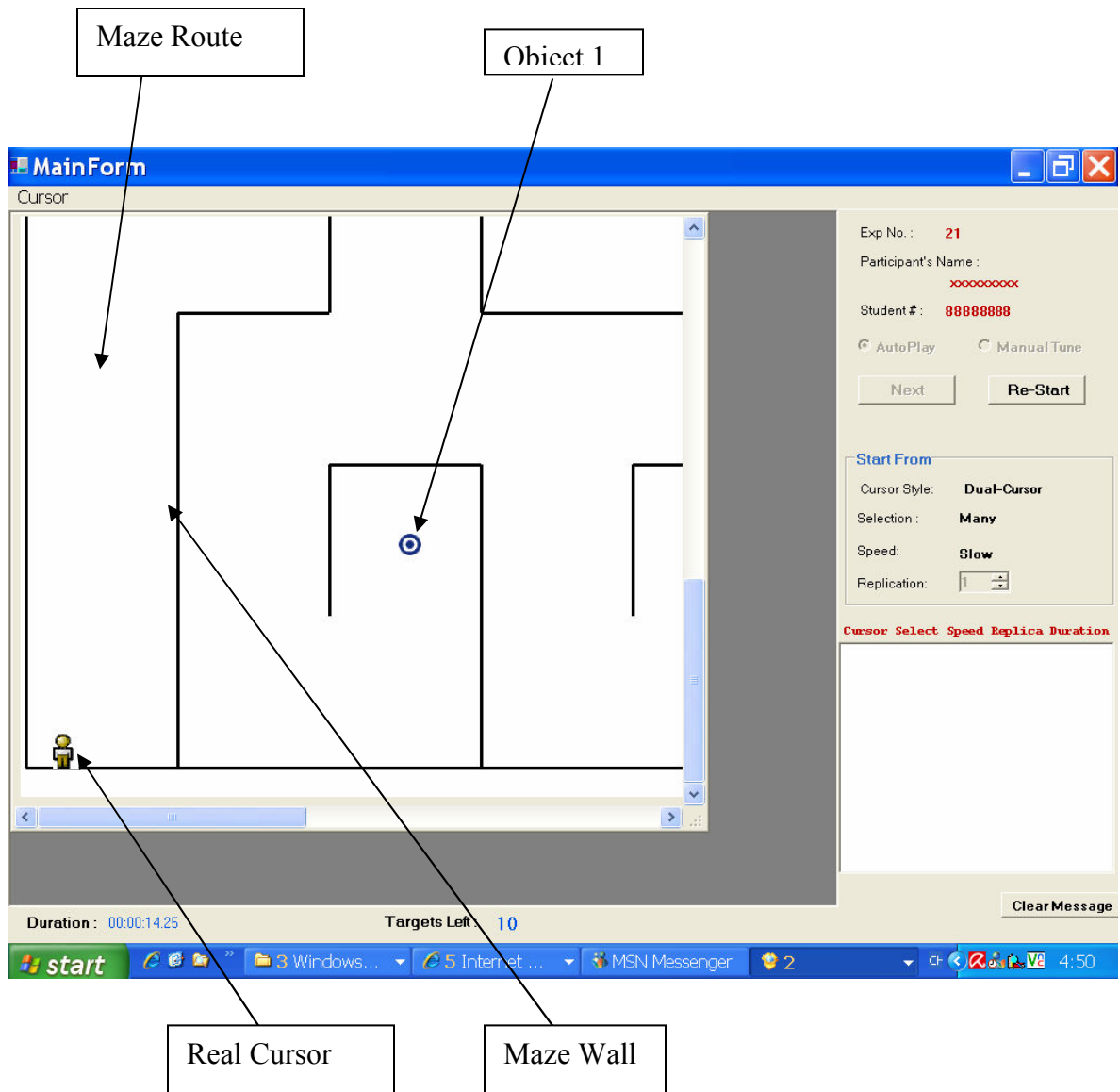
Figure 8-1: Initial position before triggering the dual-cursor technique. Only the real cursor is visible. The dual cursor becomes visible only when the user depresses a button on the input device.
