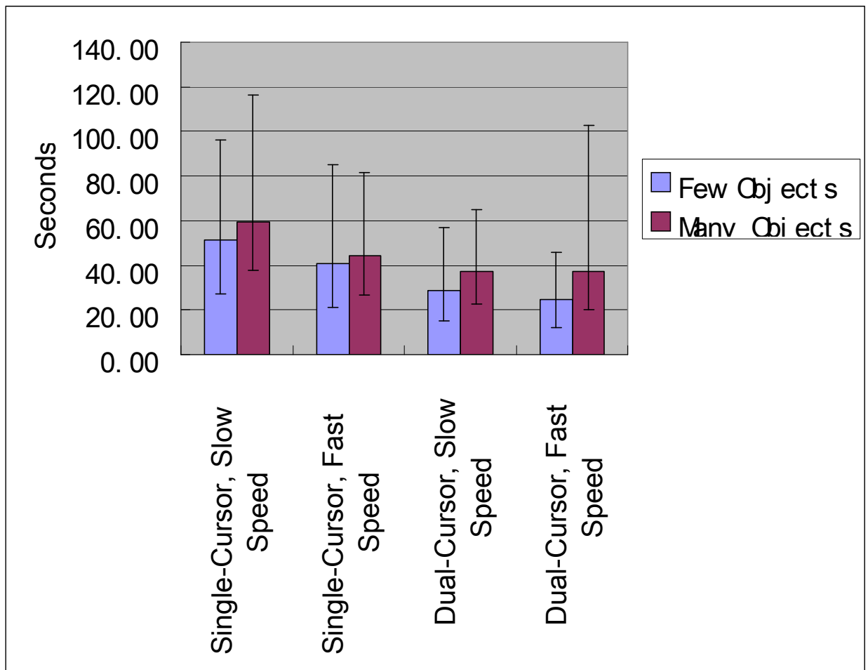
Chart 3. Chart of experiment 3 results
