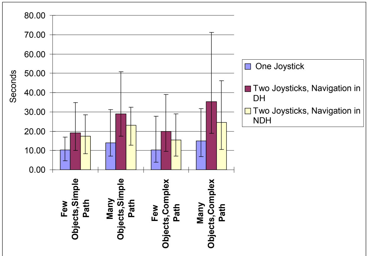
Chart 1: Summary of results. Unimanual outperformed both types of bimanual. However, comparing both bimanual techniques we observe that Guiard's theory is upheld.
