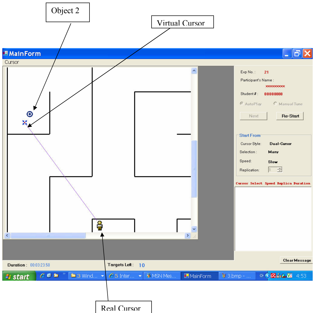
Figure 8-4: Dual-cursor initiated toward a new target.
