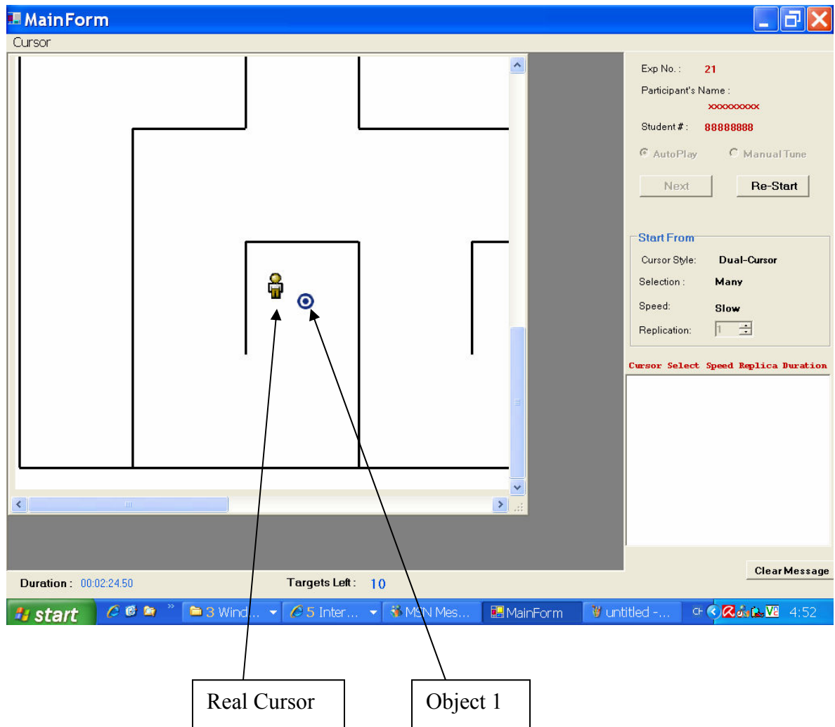
Figure 8-3: Once the user is satisfied with the location of interest, he/she can trigger a teleportation which brings the real cursor to the vicinity of the virtual cursor. In this manner the user can jump around the scene.
