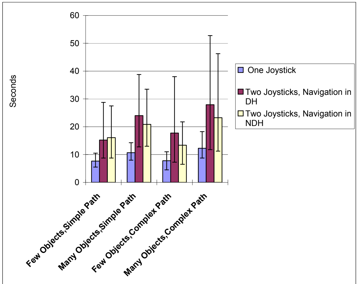
Chart 2: Summary of results. Unimanual outperformed both types of bimanual. However, comparing both bimanual techniques we observe that Guiard's theory is upheld.
