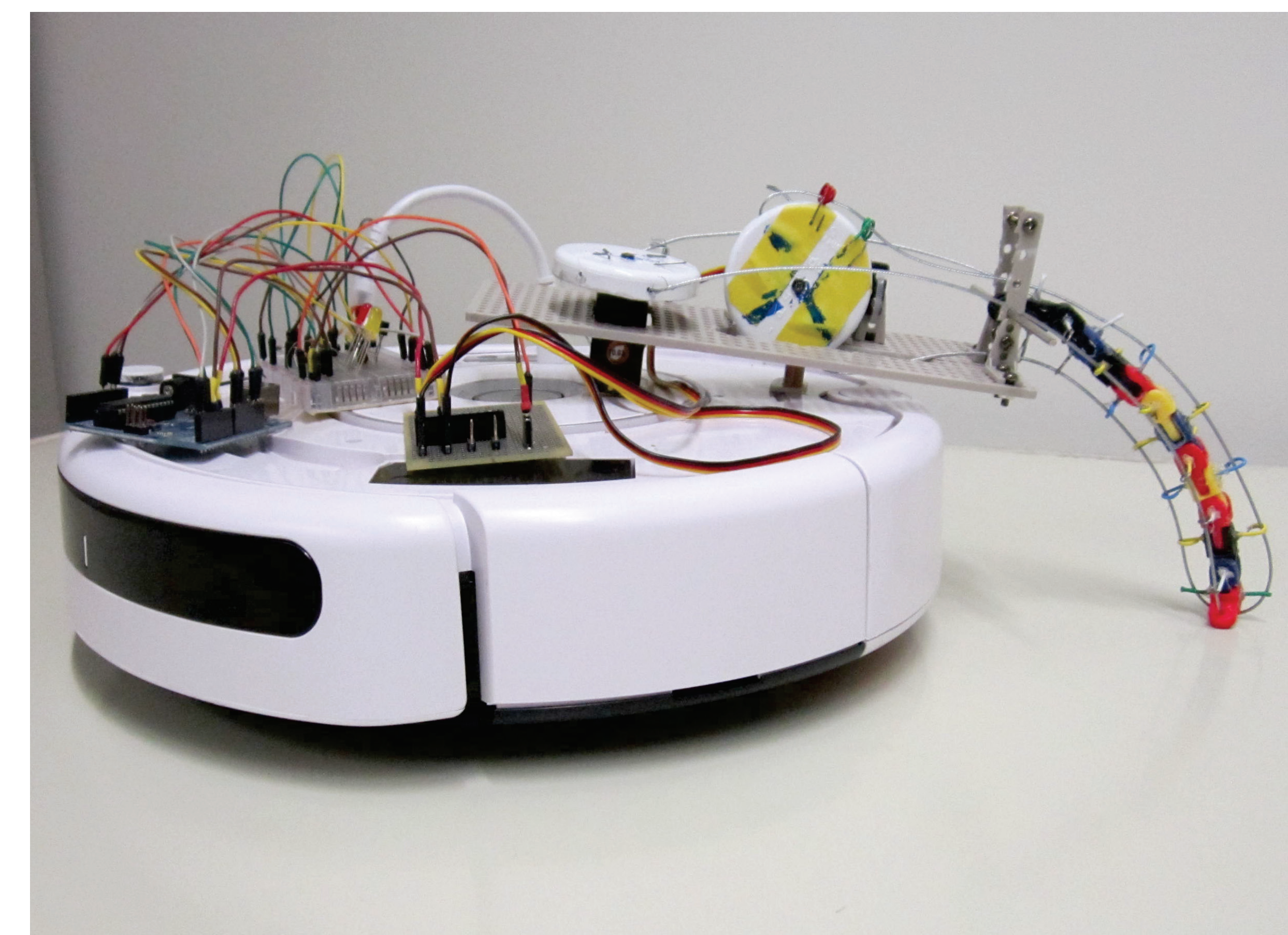
tail lowered - scared stuck in between objects
