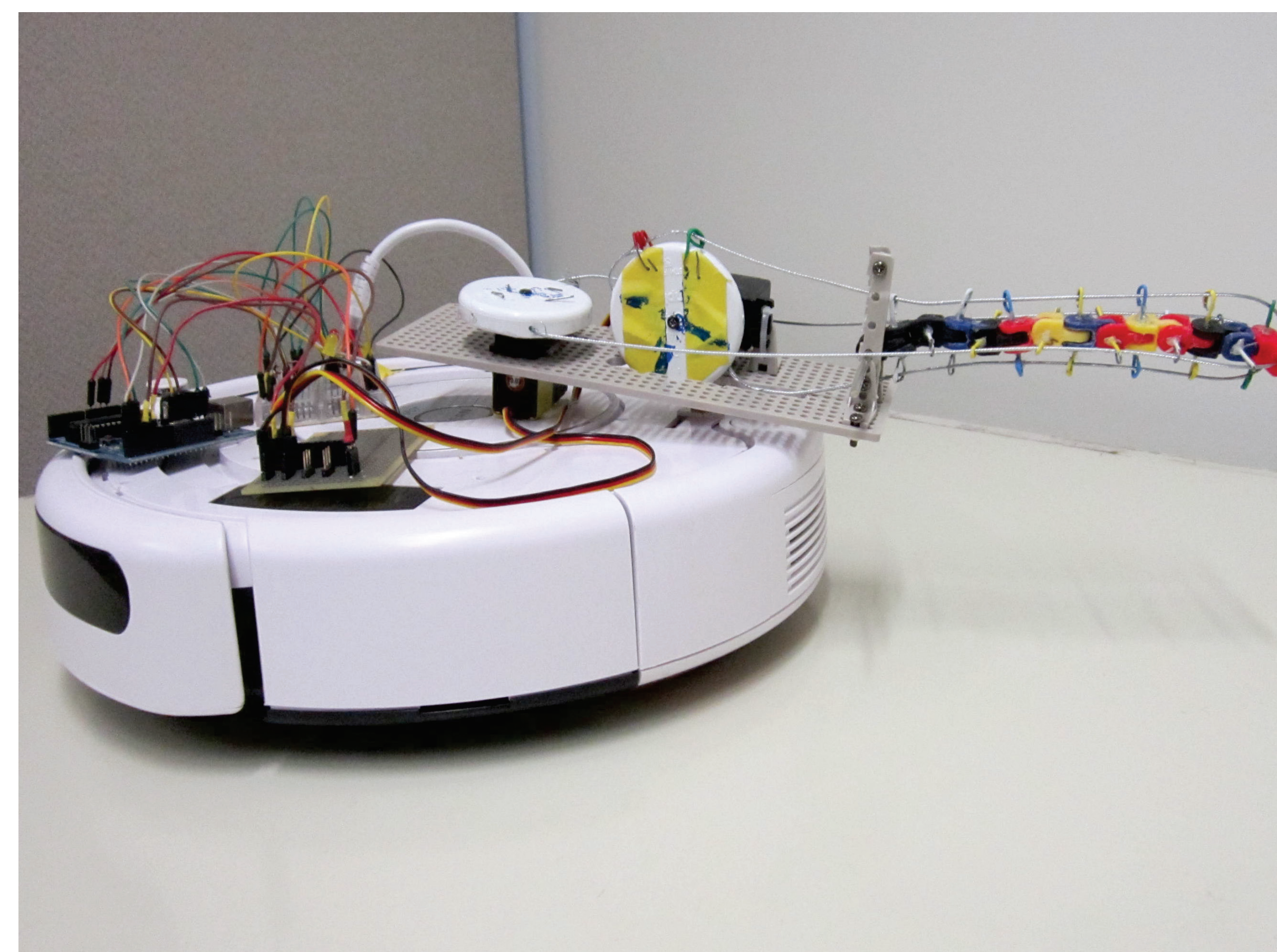
tail straight - courteous bumping into people and objects
